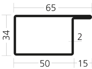
WP 3450/15 L /5400-0010-57184
