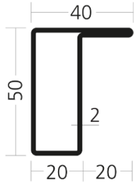
WP 5020/20 L /5400-0010-5965
