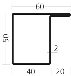
WP 5040/20 L /5400-0010-2144
