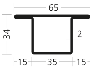
WP 3435/15 T /5400-0010-54160
