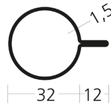
WP 32/12 R /5400-0010-R3212
