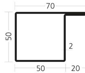
WP 5050/20 L /5400-0010-L505020
