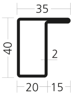
WP 4020/15 L /5400-0010-54232
