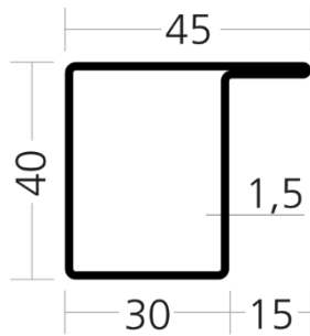
WP 4030/15 L /5400-0010-L403015
