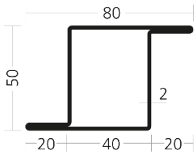
WP 5040/20 Z /5400-0010-Z504020
