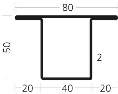
WP 5040/20 T /5400-0010-2140
