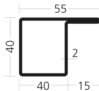
WP 4040/15 L /5400-0010-5340
