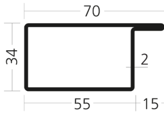
WP 3455/15 L /5400-0010-53101
