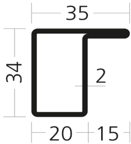
WP 3420/15 L /5400-0010-54235
