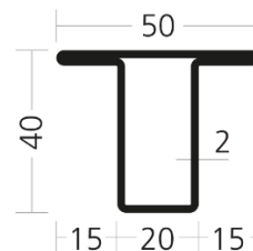
WP 4020/15 T /5400-0010-53209
