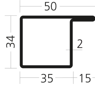
WP 3435/15 L /5400-0010-53100
