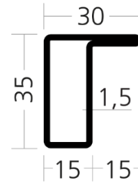
WP 3515/15 L /5400-0010-L351515
