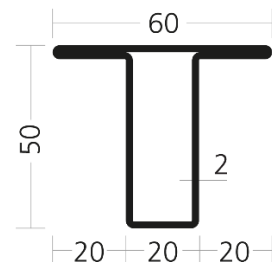
WP 5020/20 T /5400-0010-5964
