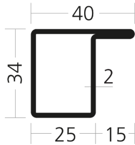
WP 3425/15 L /5400-0010-54234
