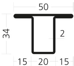
WP 3420/15 T /5400-0010-5722
