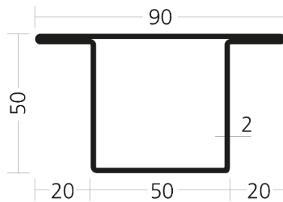
WP 5050/20 T /5400-0010-T505020
