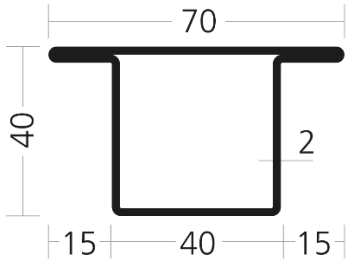
WP 4040/15 T /5400-0010-53162
