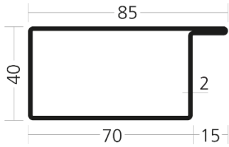
WP 4070/15 L /5400-0010-5966
