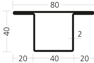
WP 4040/20 T /5400-0010-T404020
