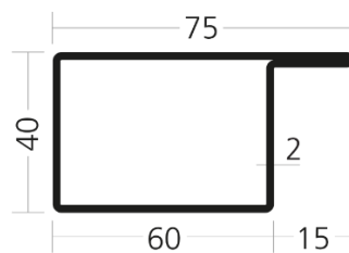
WP 4060/15 L /5400-0010-6291
