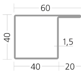
WP 4040/20 L /5400-0010-L404020
