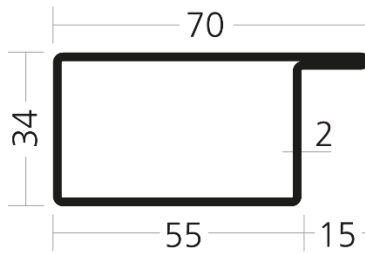
WP 3455/15 L /5400-0010-53101
